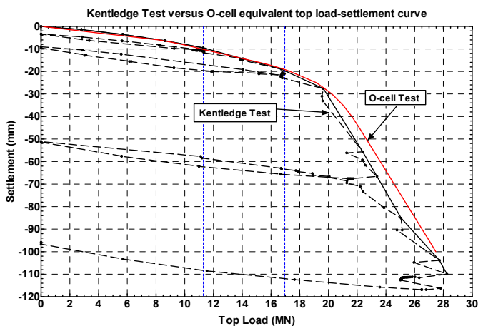
Fig 3 Comparison between top down and bi-directional
