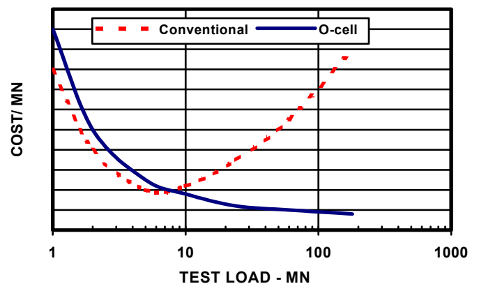
Fig 4 COMPARISON OF LOAD TESTING COSTS CONVENTIONAL VS. O-CELL
