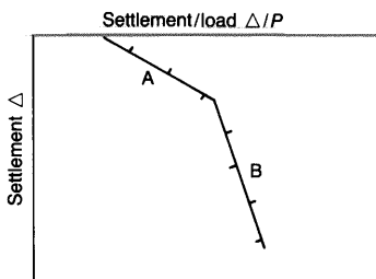
Fig. 1. Relationship of settlement and settlement/load
